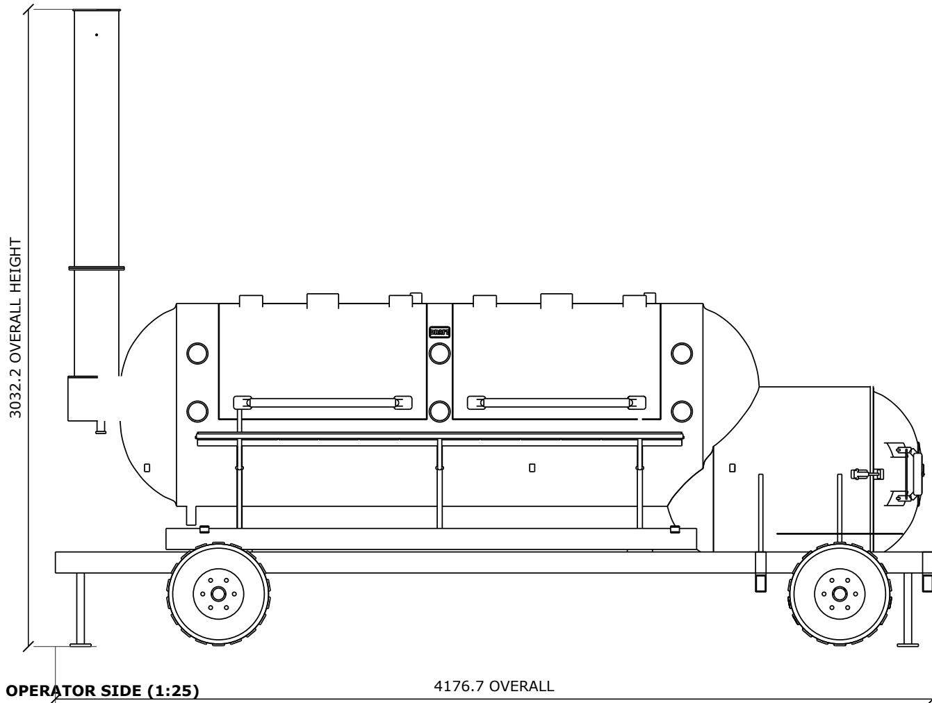
FRONT / OPERATOR SIDE (1:25)
